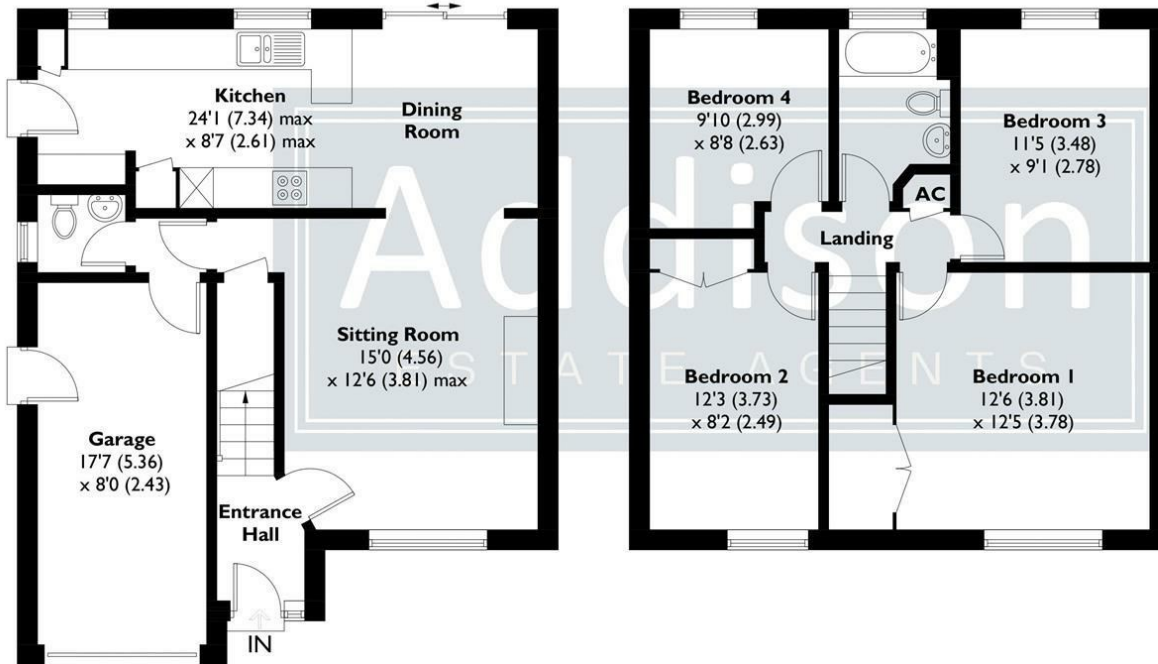
GROUND FLOOR 659 SQ FT / 61.2 SQ M
