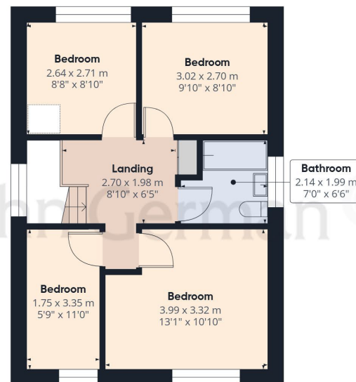
Floor 1 Building 1
