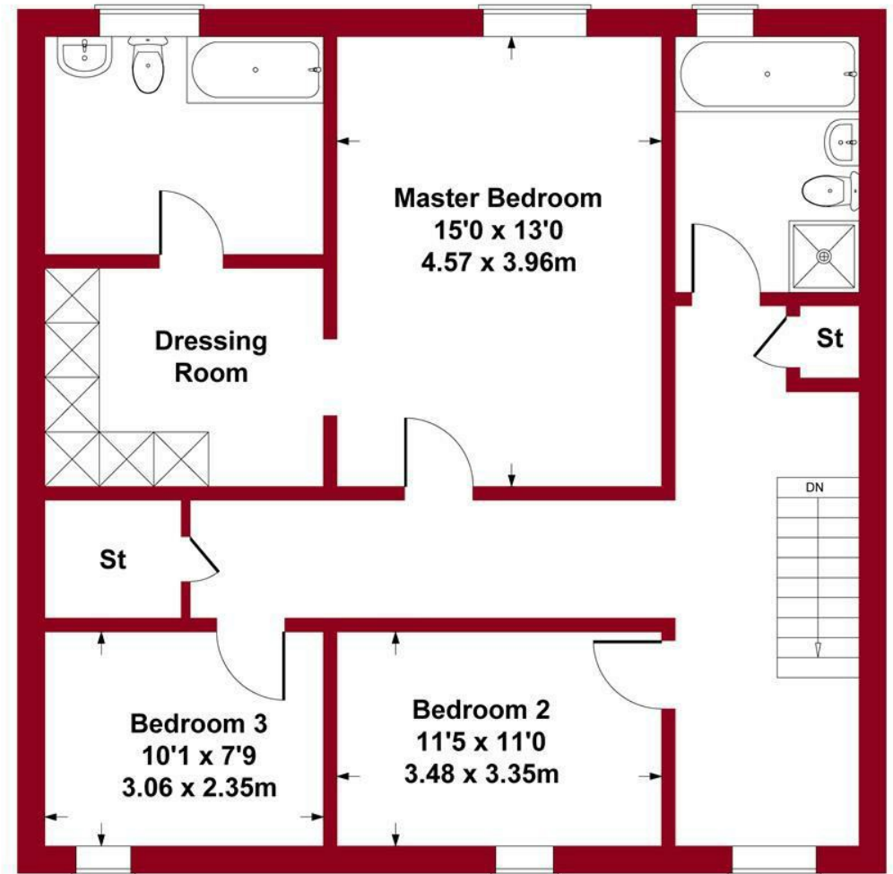
FIRST FLOOR (PLOT 2)
