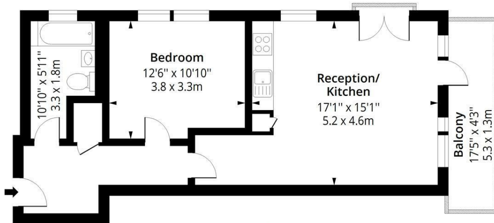
Sixth Floor Floor Area 585 Sq Ft - 54.35 Sq M
