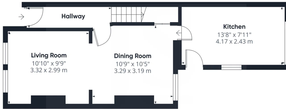
Ground Floor
