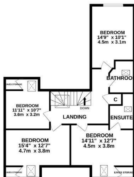
1ST FLOOR 811 sq.ft. (75.3 sq.m.) approx.
