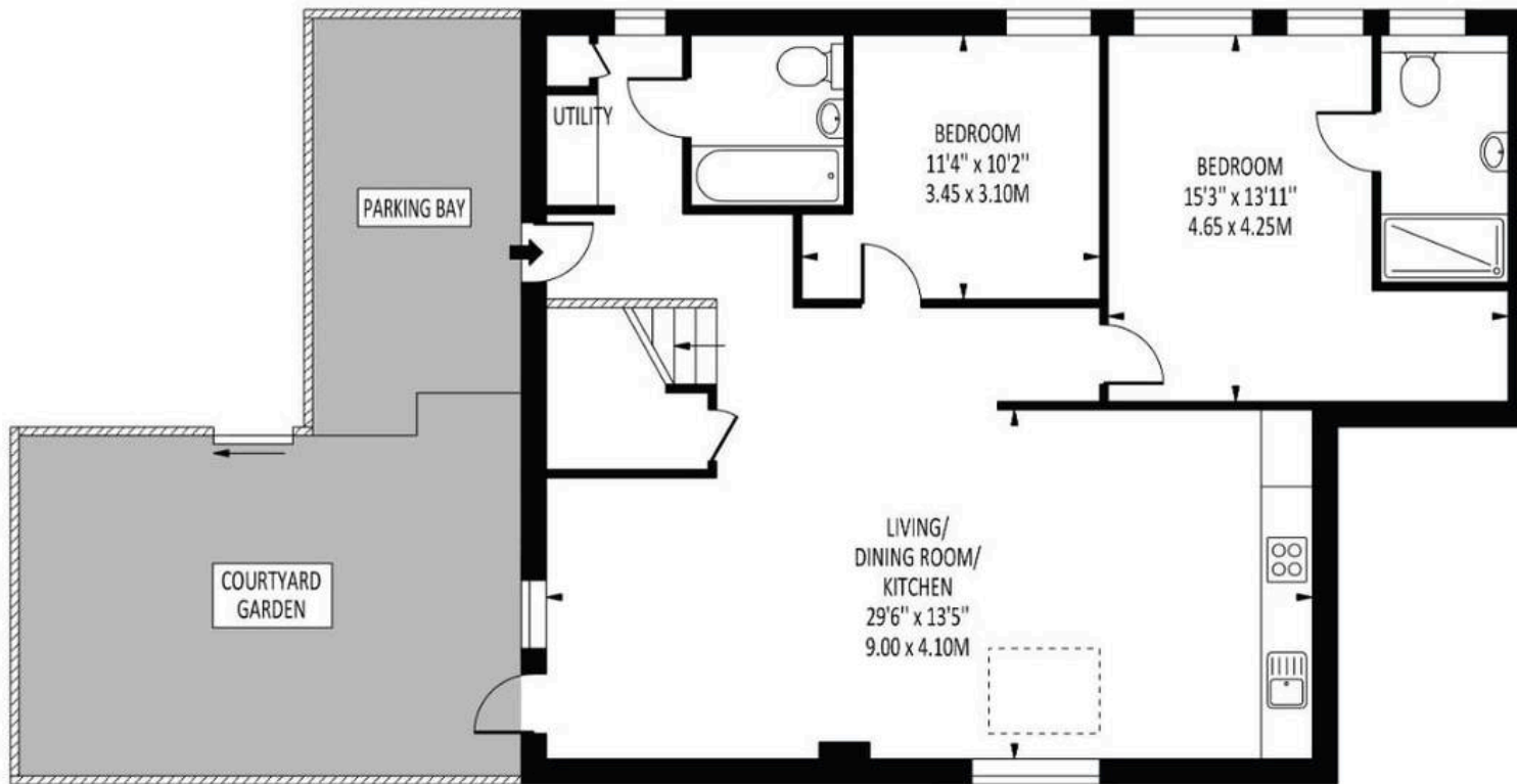
GROUND FLOOR
