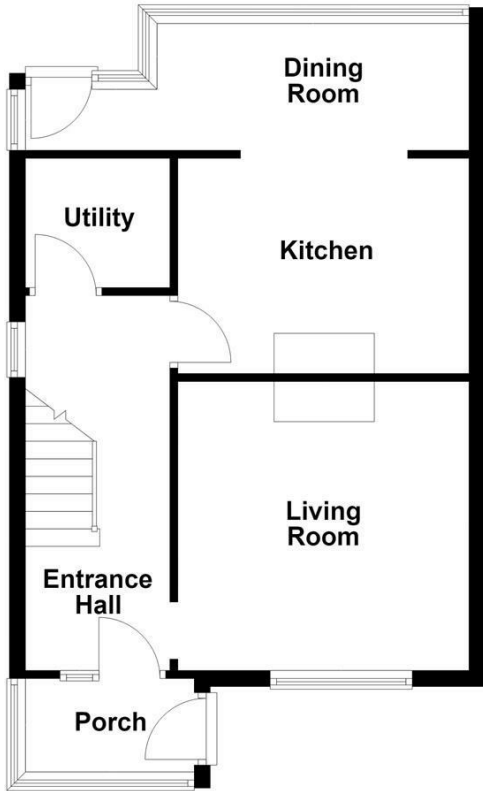
Ground Floor Approx. 45.9 sq. metres (493.9 sq. feet)
