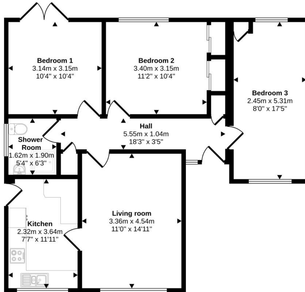
Floorplan
