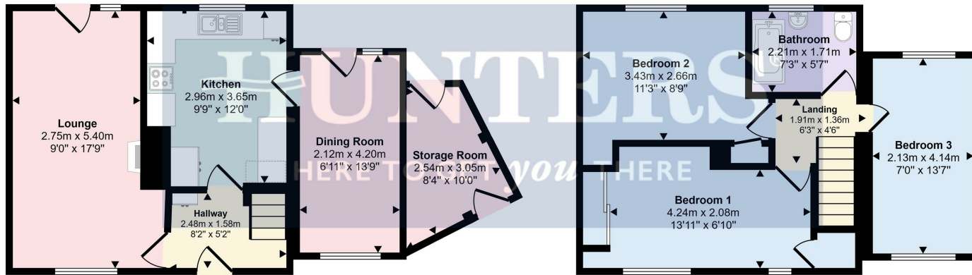
Ground Floor Approx 47 sq m / 510 sq ft
