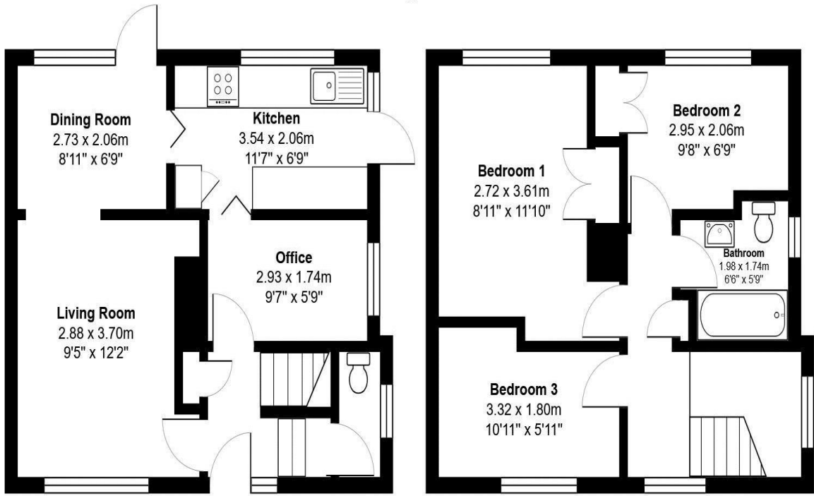
Ground Floor Area: 38.5 m 2 ... 415 ft 2
