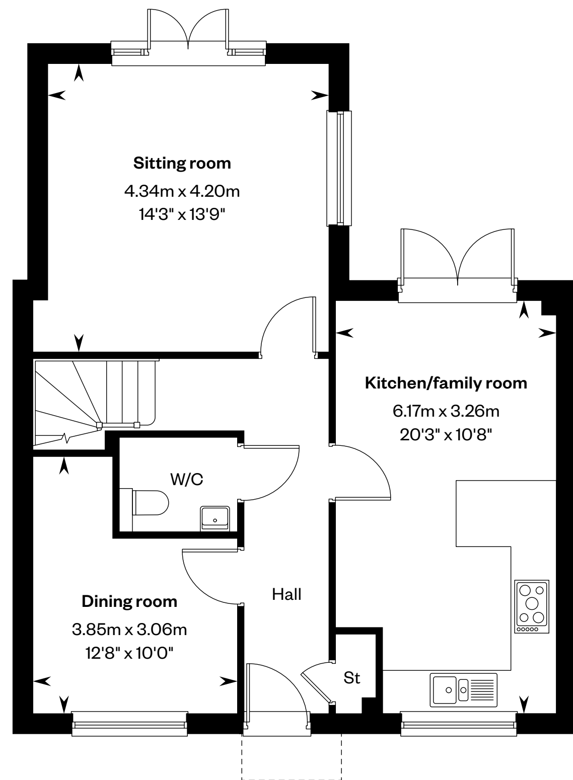
Ground floor
