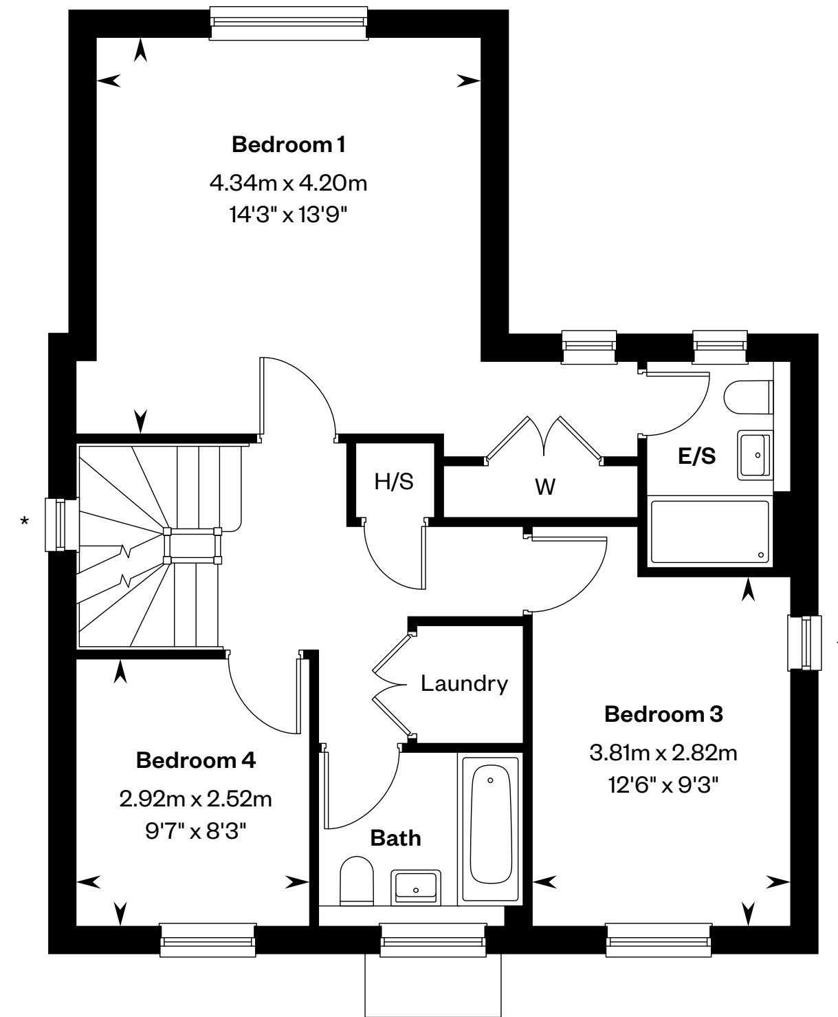
First floor
