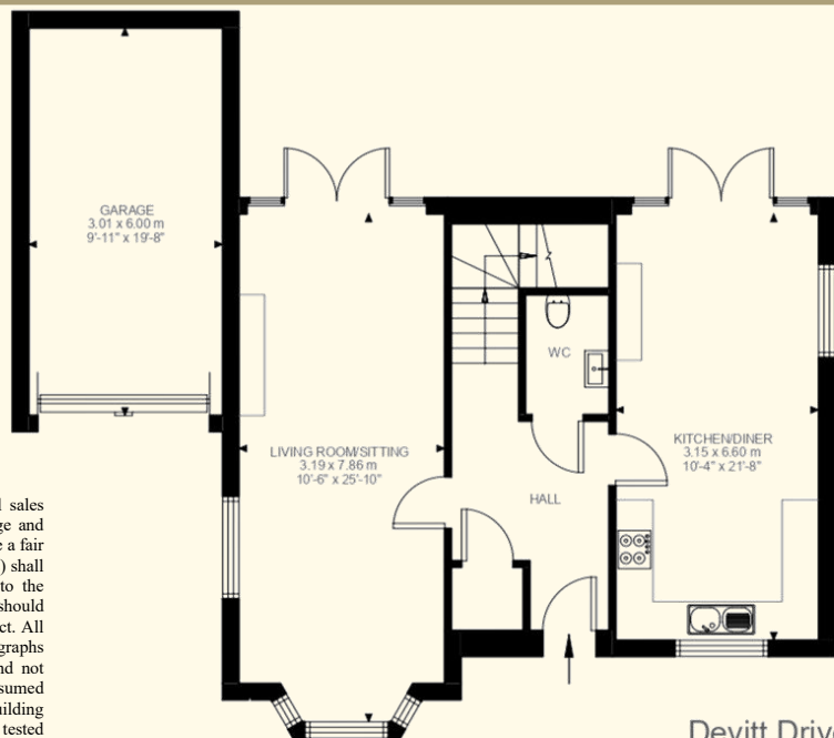
Ground Floor 673 ft²
