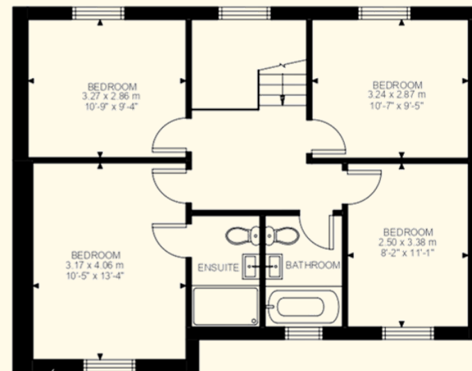
First Floor 645 ft²
