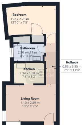
Floor 0 Building 2
