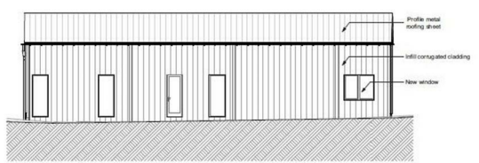
North-West Elevation - Scale 1:100
