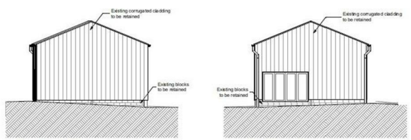
South-West Elevation - Scale 1:100 North-East Elevation - Scale 1:100
