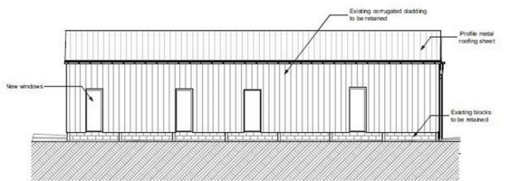
South-East Elevation - Scale 1:100
