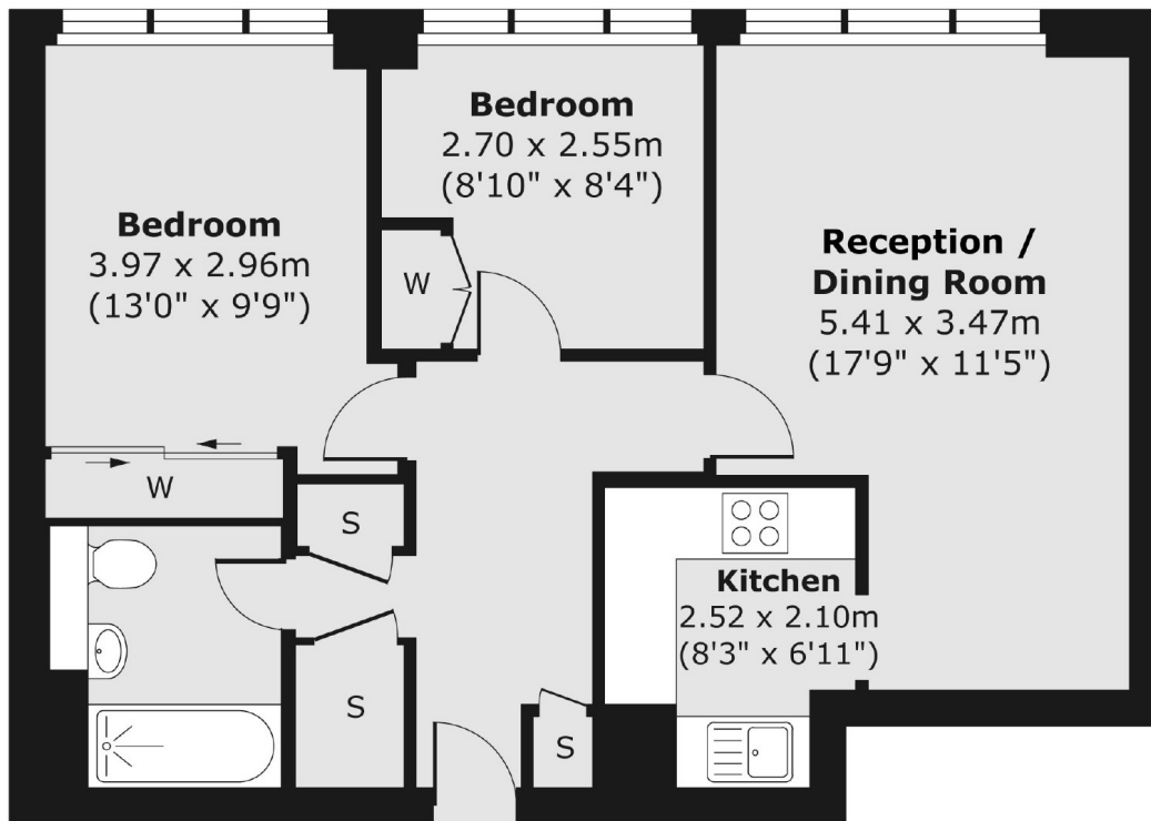
Third Floor
