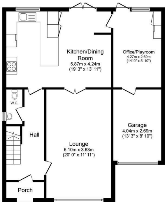
Floor area 84.8 sq.m. (912 sq.ft.)
