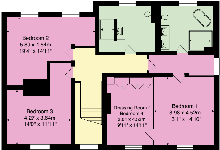
Main House - First Floor Area: 122.8 m 2 ... 1322 ft 2
