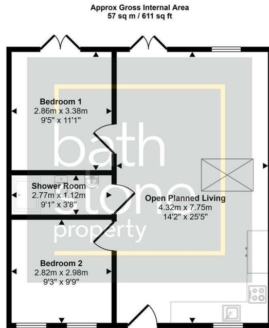
Floorplan
