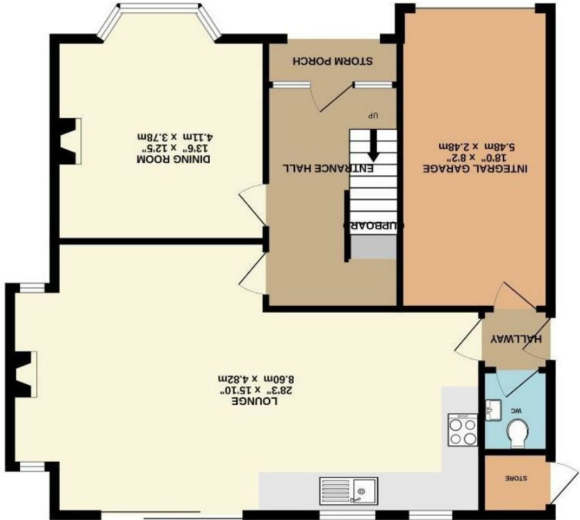
GROUND FLOOR 872 sq.ft. (81.0 sq.m.) approx.
