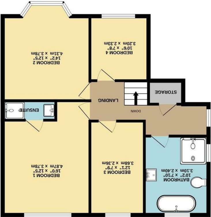
1ST FLOOR 745 sq.ft. (69.2 sq.m.) approx.
