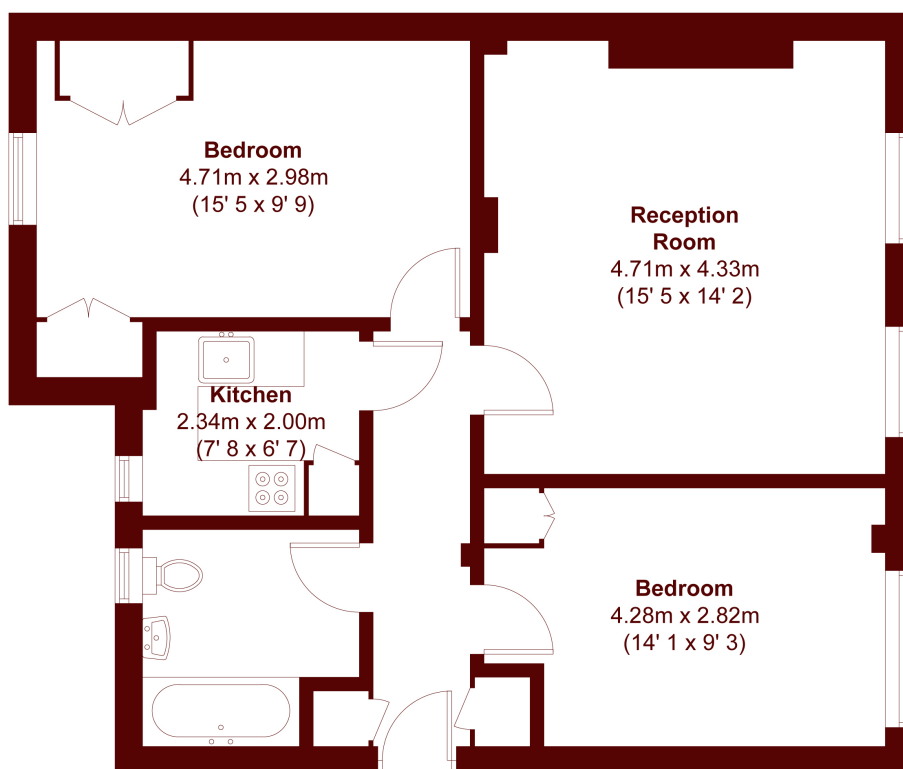
Second Floor
