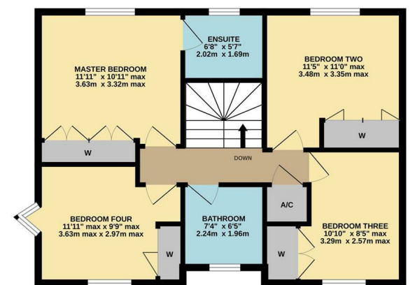
TOTAL FLOOR AREA: 1282 sq.ft. (119.1 sq.m.) approx.
