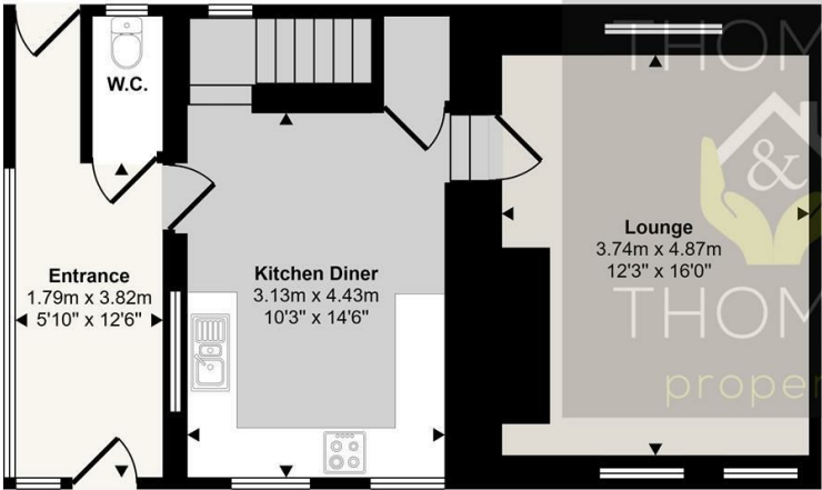
Ground Floor Approx 54 sq m / 583 sq ft
