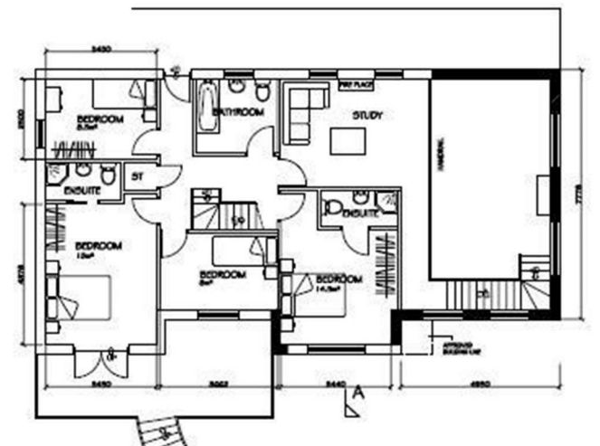
GROUND FLOOR 100.00m 2 1,076.41sqft
