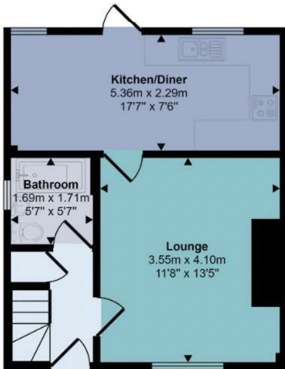
Ground Floor Approx 35 sq m / 374 sq ft
