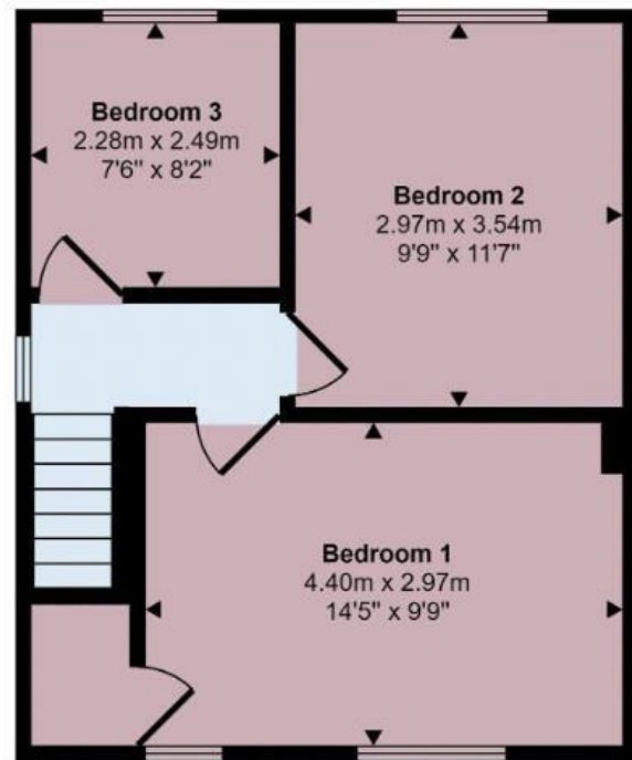
First Floor Approx 36 sq m / 391 sq ft
