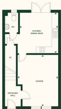
GROUND FLOOR
