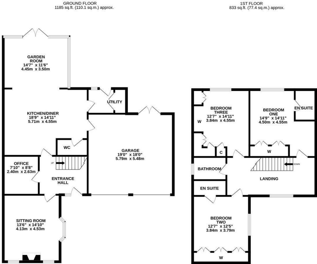
TOTAL FLOOR AREA : 2018 sq.ft. (187.4 sq.m.) approx. Whilst every attempt has been made to ensure the accuracy of the floorplan contained here, measurements of doors, windows, rooms and any other items are approximate and no responsibility is taken for any error, omission or mis-statement. This plan is for illustrative purposes only and should be used as such by any prospective purchaser. The services, systems and appliances shown have not been tested and no guarantee as to their operability or efficiency can be given. Made with Metropix ©2026
