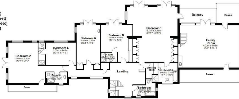
First Floor Approx. 273.5 .sq.metres (2944.4 sq. feet)
