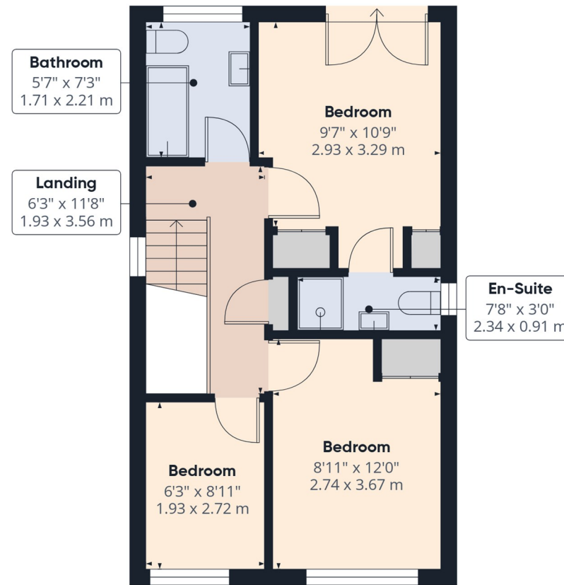
Floor 1 Building 1
