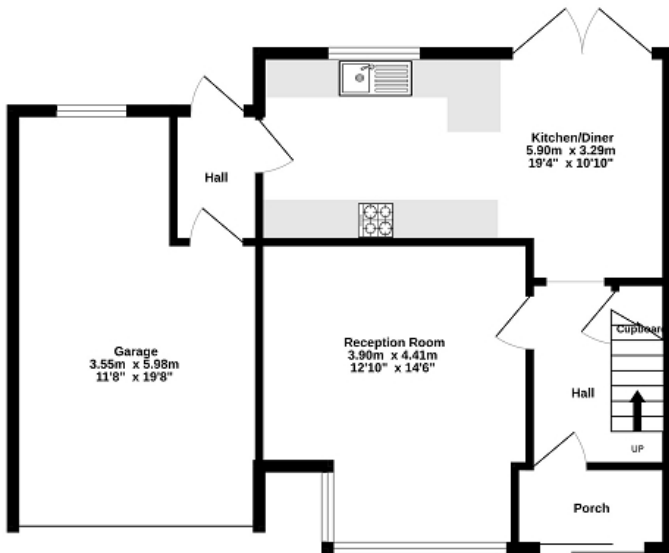
Ground Floor 62.2 sq.m. (669 sq.ft.) approx.
