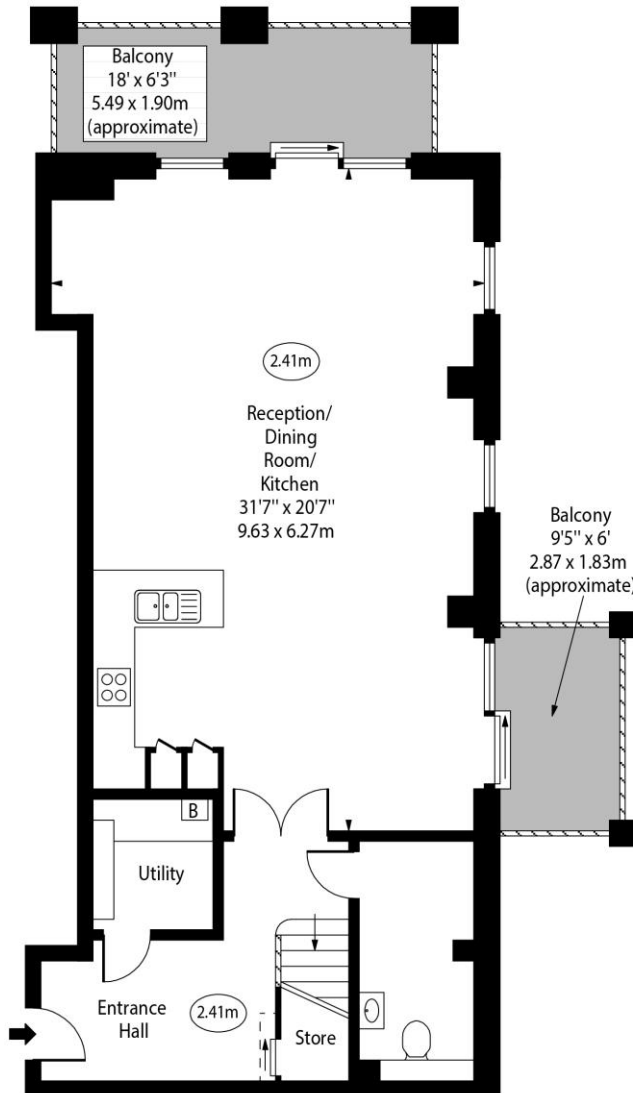
Eighteenth Floor
