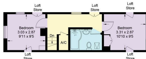
First Floor
