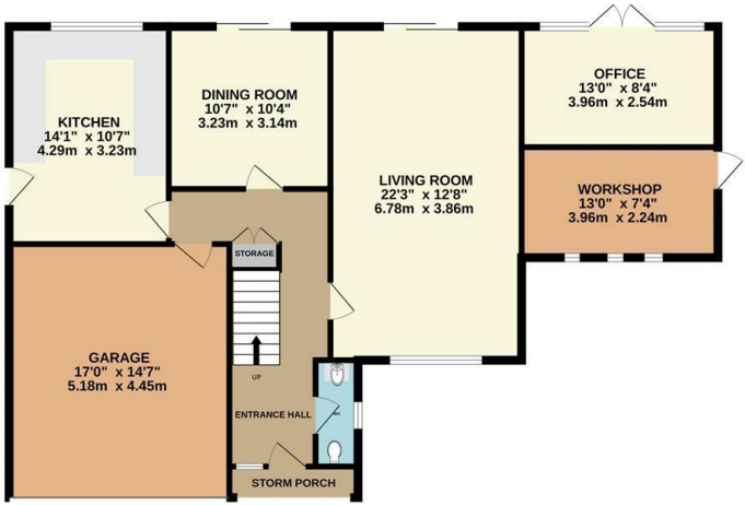
GROUND FLOOR 1173 sq.ft. (108.9 sq.m.) approx.
