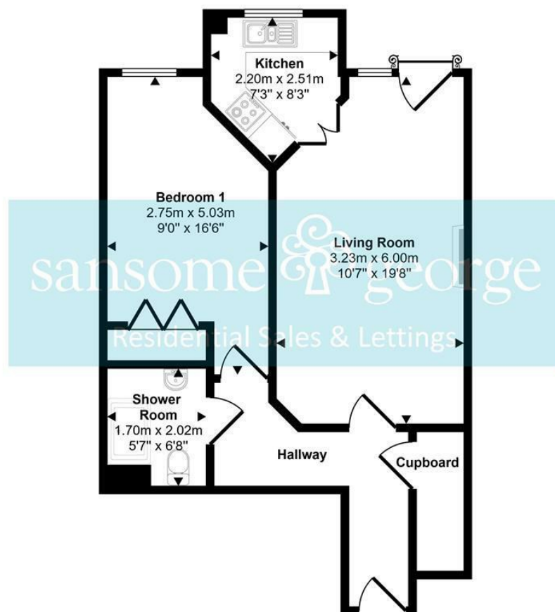
Floorplan
