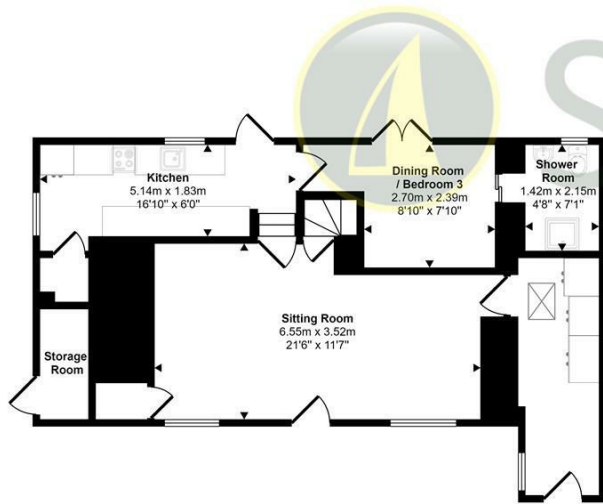
Ground Floor Approx 63 sq m / 681 sq ft
