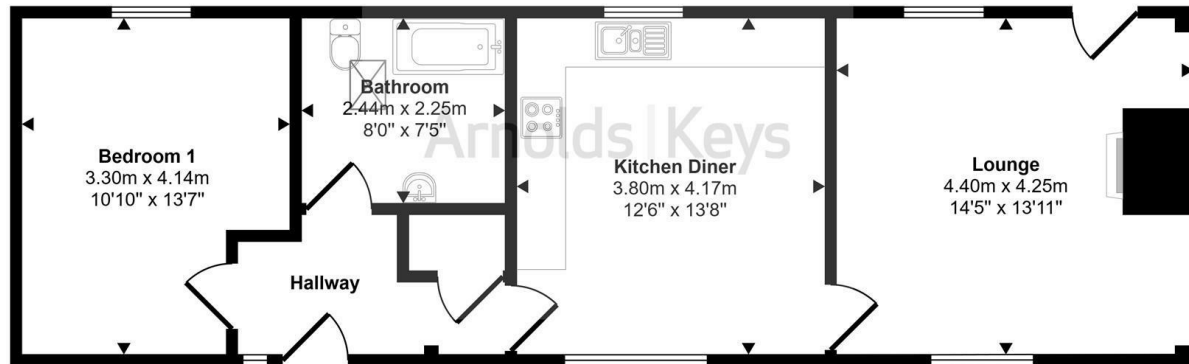
Floorplan
