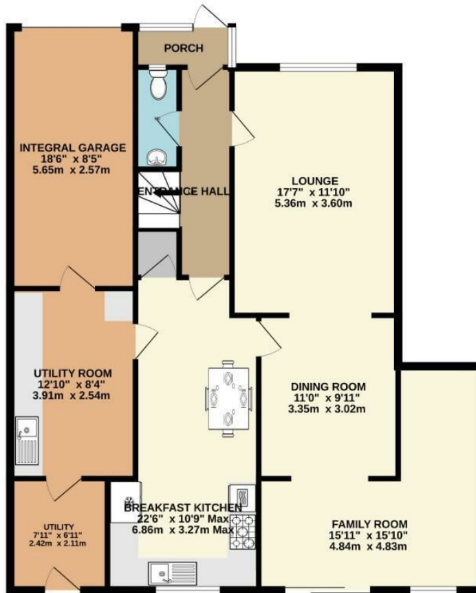
GROUND FLOOR 1161 sq.ft. (107.8 sq.m.) approx.
