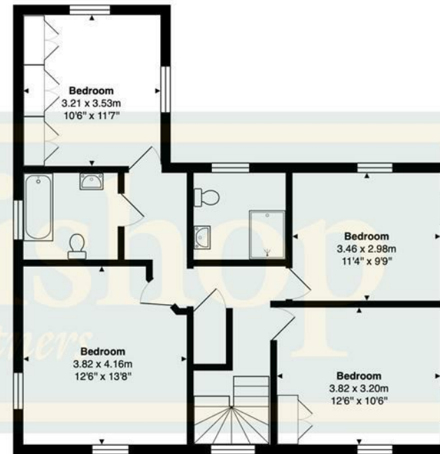
First Floor Area: 73.7 m 2 ... 793 ft 2
