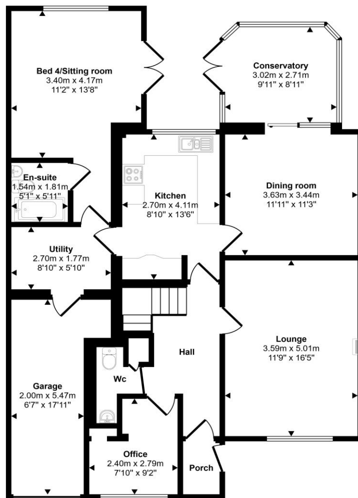
Ground Floor Approx 111 sq m / 1199 sq ft
