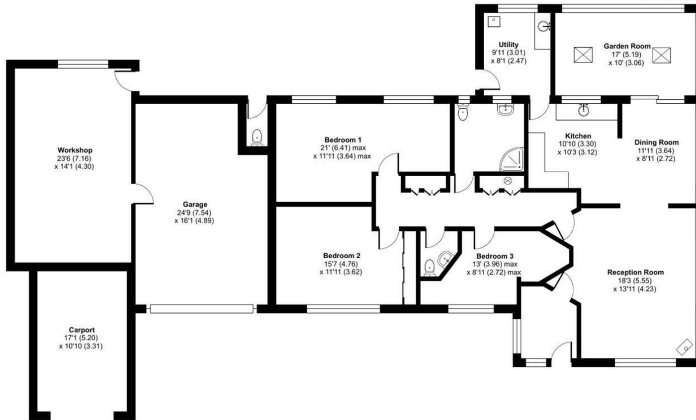
GROUND FLOOR
