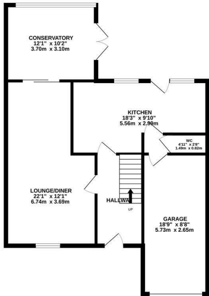
GROUND FLOOR 780 sq.ft. (72.4 sq.m.) approx.
