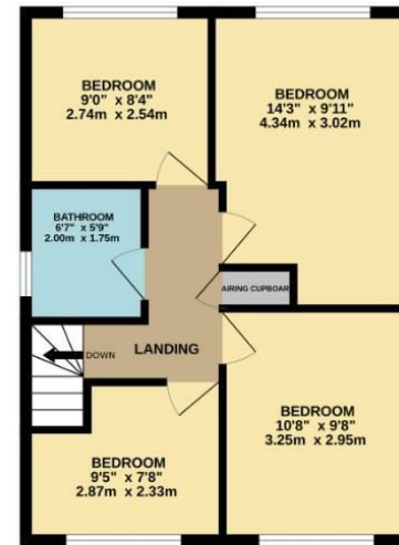
1ST FLOOR 477 sq.ft. (44.3 sq.m.) approx.
