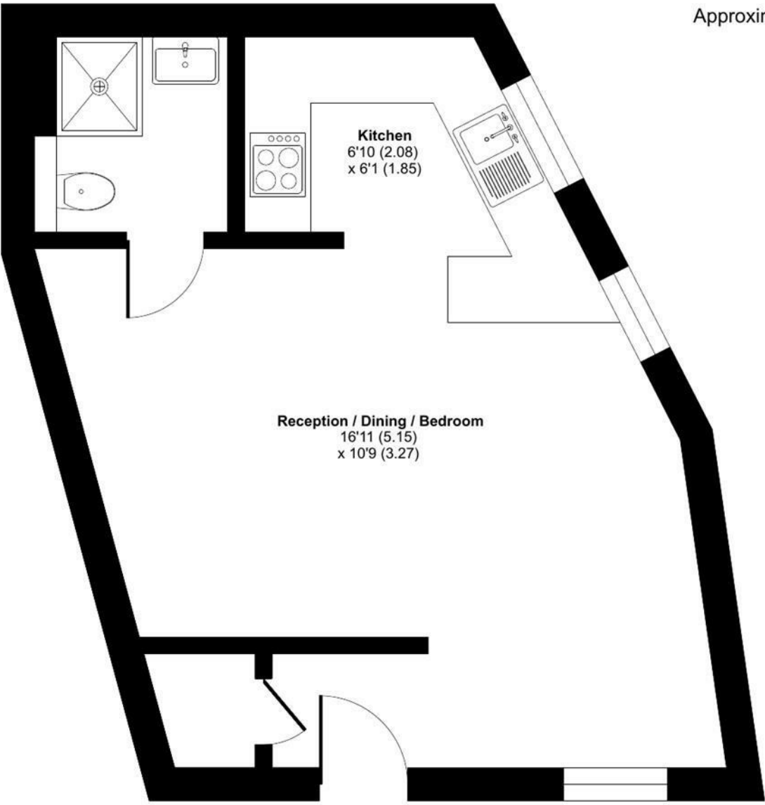
GROUND FLOOR
