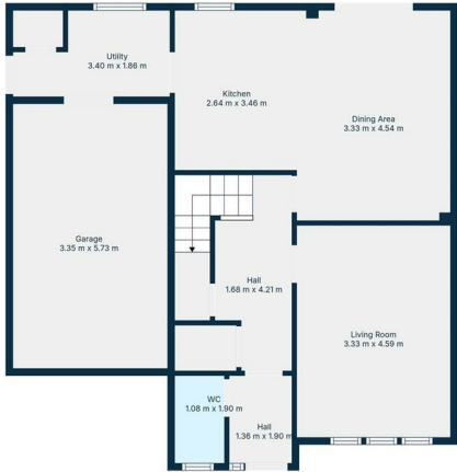
TOTAL: 138 m 2 Ground floor: 58 m 2 , 1st floor: 80 m 2 EXCLUDED AREAS: GARAGE: 19 m 2 , UTILITY: 5 m 2 , STAIRWELL: 4 m 2 , WALLS: 14 m 2 Floor Plan Created By CalcuApp. Measurements Deemed Highly Reliable But Not Guaranteed.
