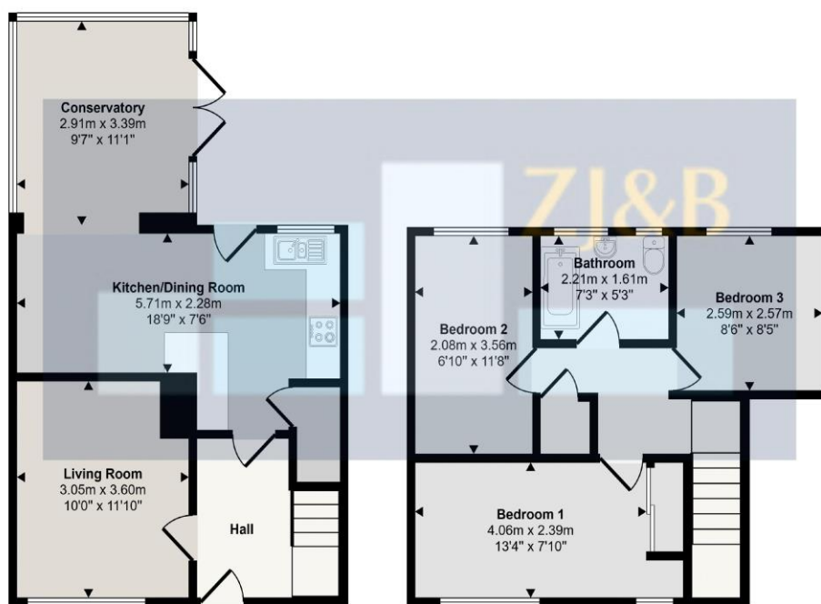
Ground Floor Approx 45 sq m / 480 sq ft
