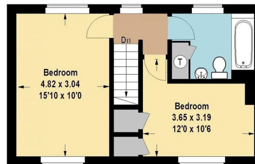
First Floor Approx Internal Floor Area 395 sq ft (36.7 sq m)
