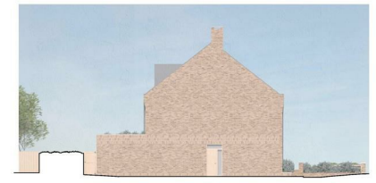
PROPOSED NORTH ELEVATION
