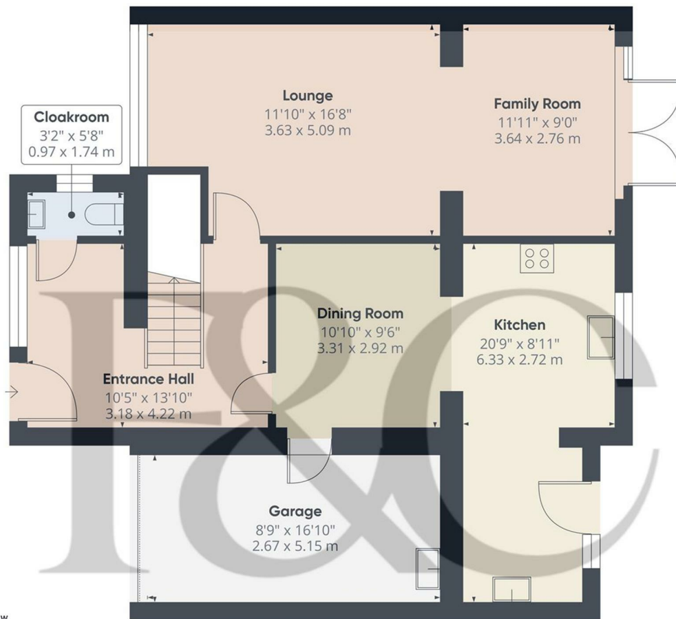
Floor 0 Building 1
