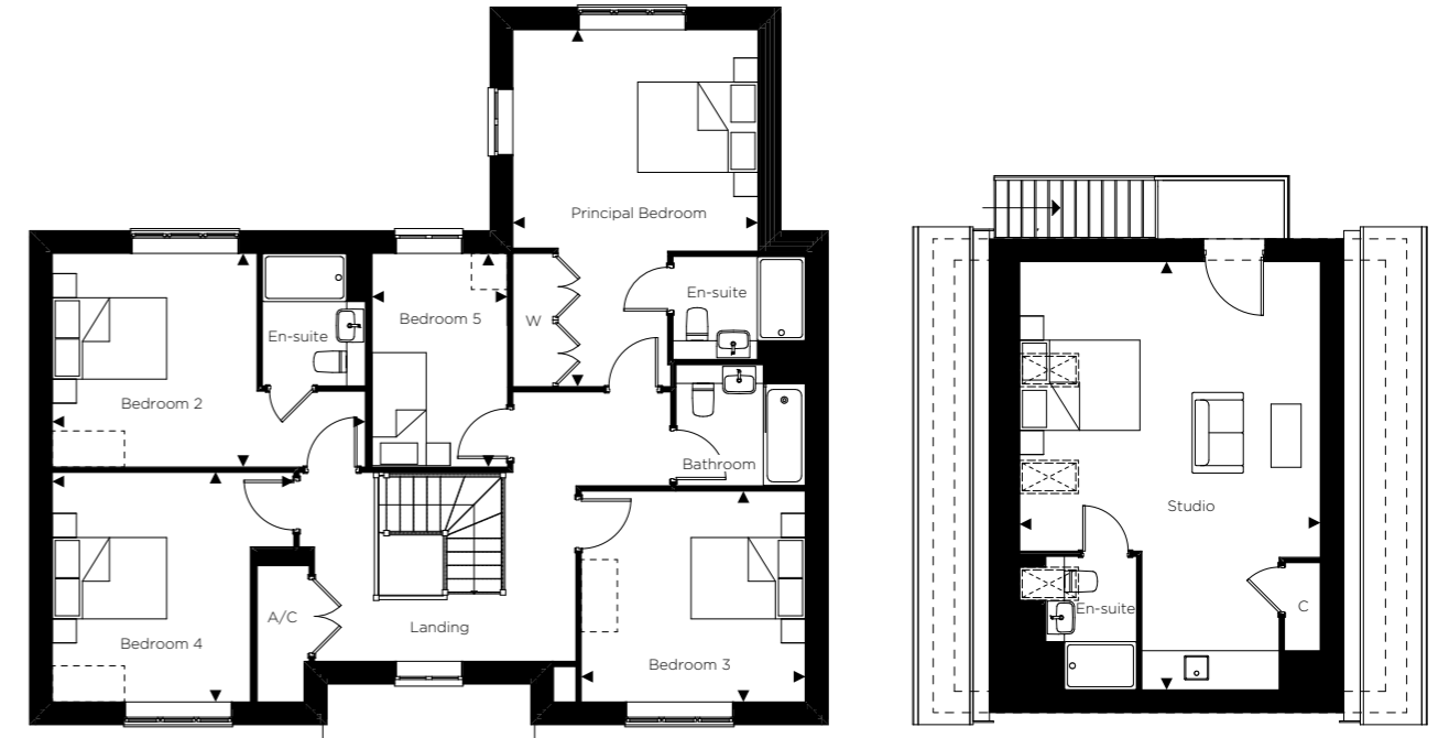
FIRST FLOOR STUDIO OVER GARAGE
