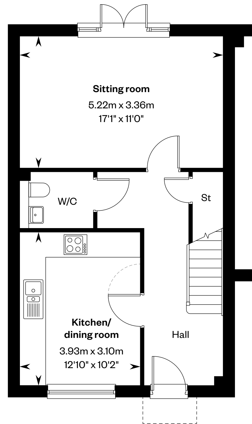
Ground floor
